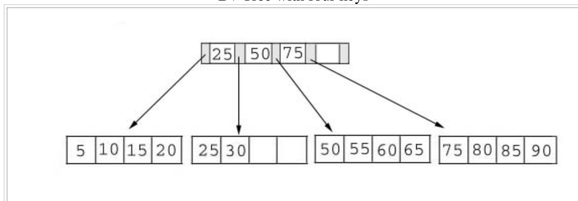
B+ Tree with four keys
